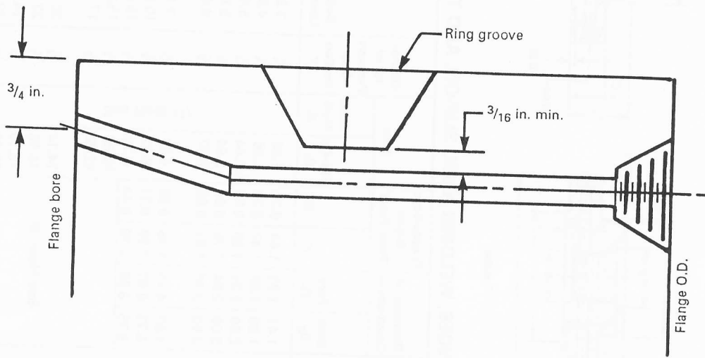
FIG. 3 ANGULAR METER TAP FOR RTJ FLANGES
